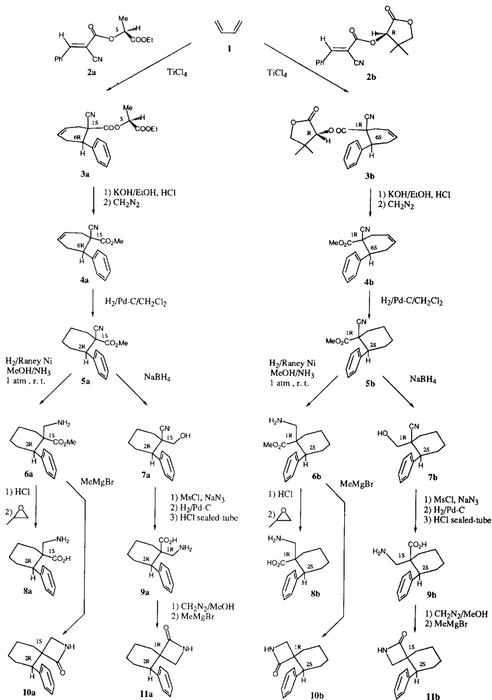
Scheme 1
